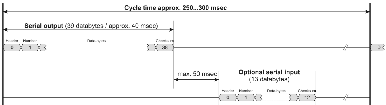
Timing: Serial Data Protocol
