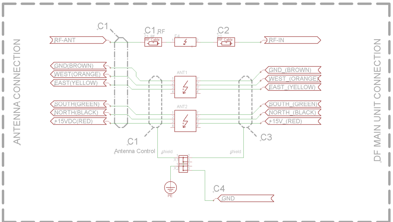
LINE PROTECTION FOR MAST INTEGRATION
